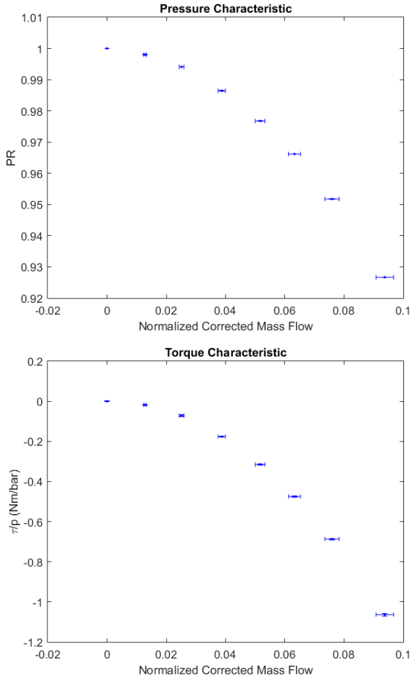
Figure 4 Experimental pressure and torque characteristics for locked rotor case.
