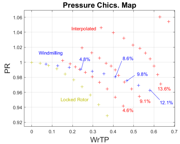
Figure 9 Interpolated low speed characteristics using windmilling line.
