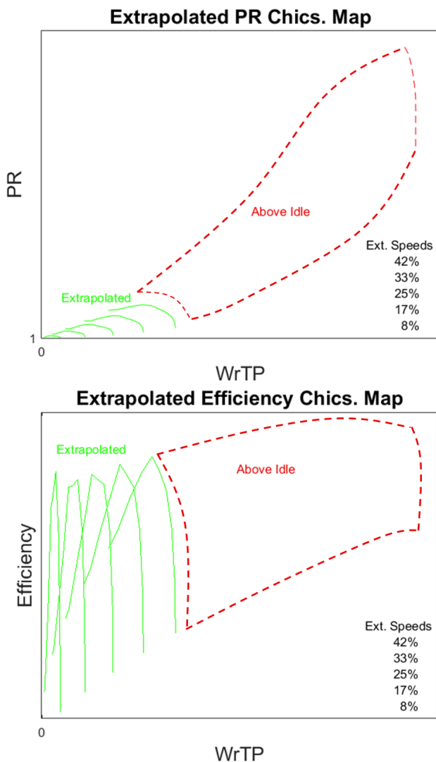
Figure 6 Extrapolated M250 axial compressor characteristics using the method in (Gaudet & Gauthier, 2007), with representative above-idle map.
