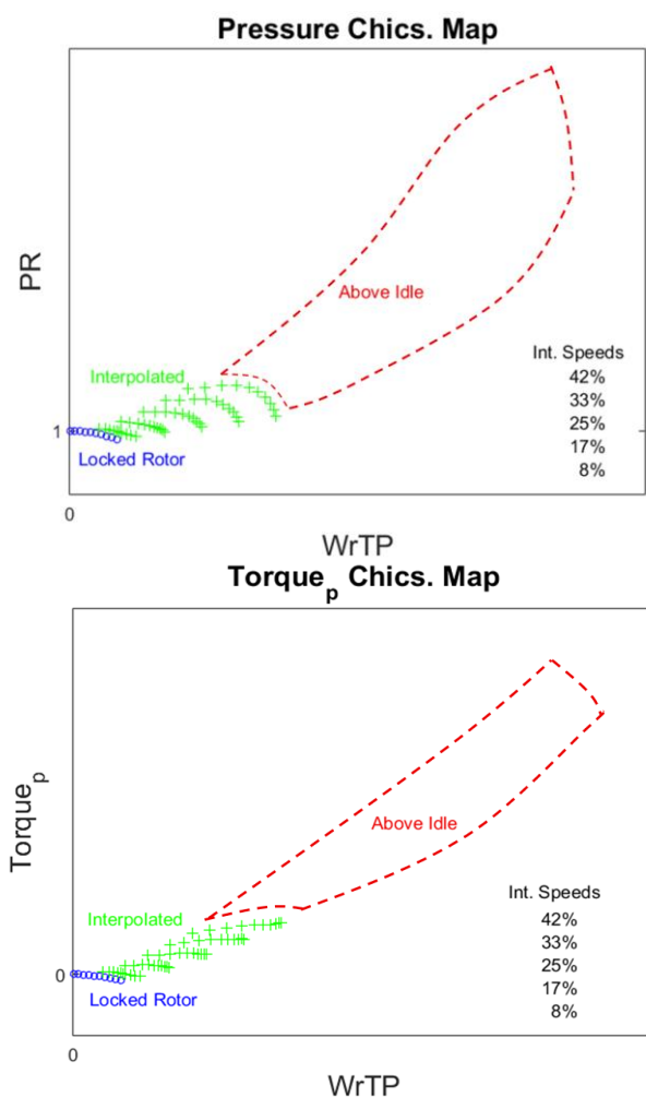
Figure 11 M250 maps after interpolation using windmilling line and representative above-idle map.
