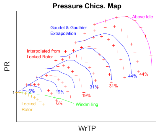
Figure 7 Comparison of interpolation and extrapolation methods for M250 sub-idle map.
