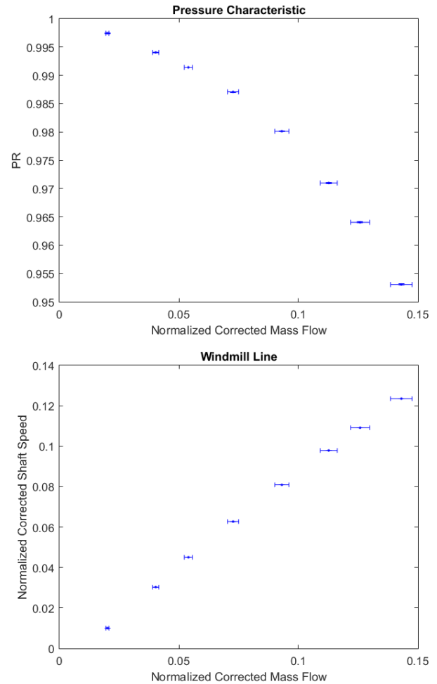
Figure 5 Experimental pressure characteristic and windmilling line for windmilling case.
