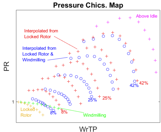
Figure 10 Comparison of interpolation methods.
